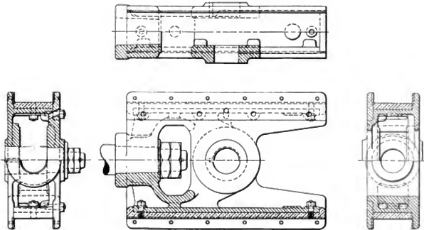
Figs. 1070-1073. Alligator Crosshead with Brass Gibs. Baldwin Locomotive Works.
